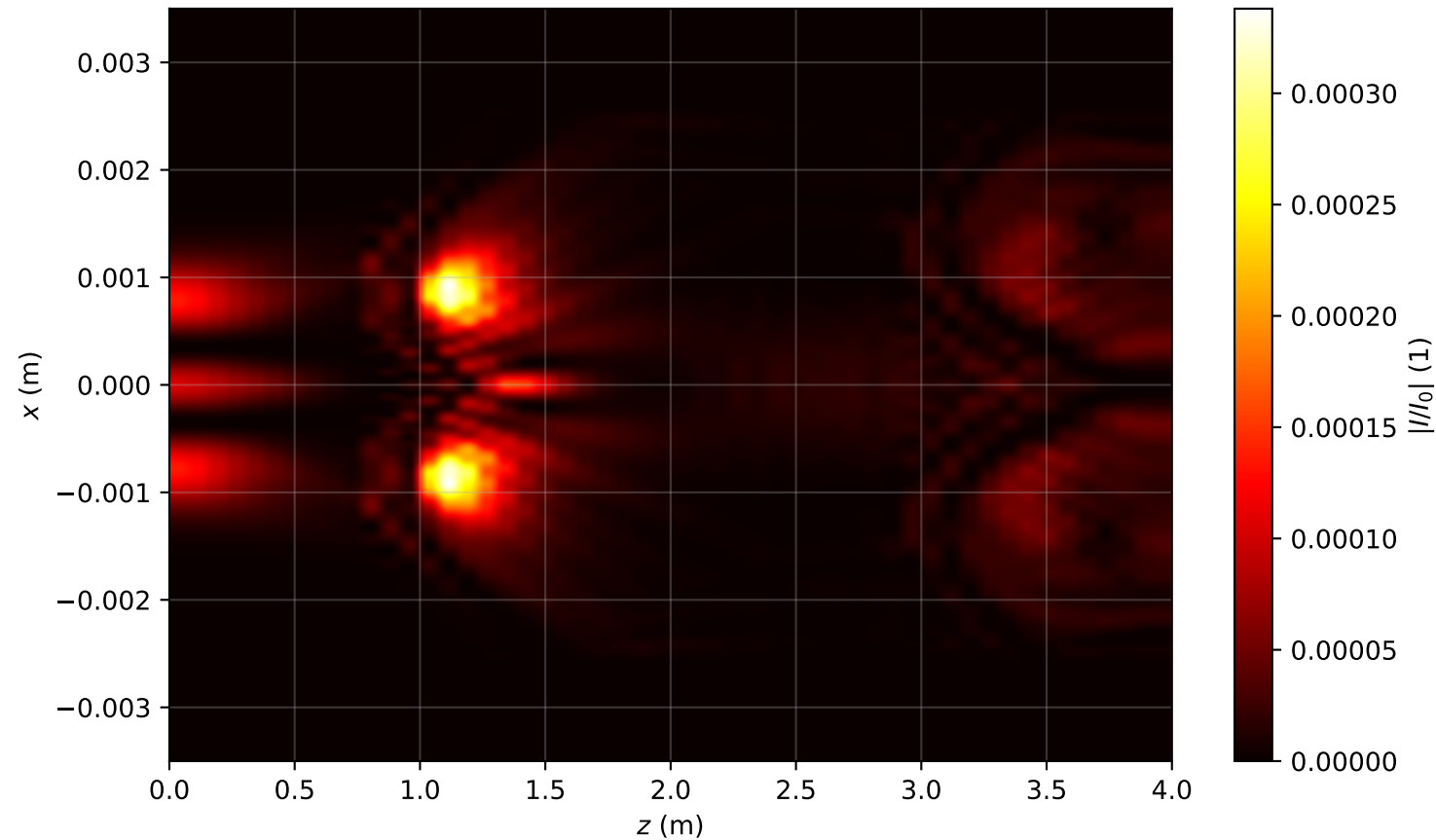
Intensity profile I(x, y = 0, z)/I_0 , P_{in}=7.0P_{cr} , artificial time
